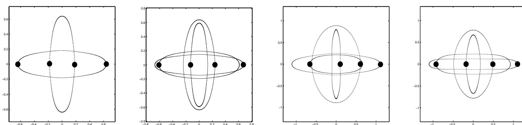
Figure 1: From left to right: The orbit in [5] with masses (m_1, m_2, m_3, m_4) = (1, 1, 1, 1) , a small perturbation with masses (0.8, 0.9, 1.1, 1) , and two large perturbation with masses (1, 2, 3, 4) and (1, 3, 4, 2) .
