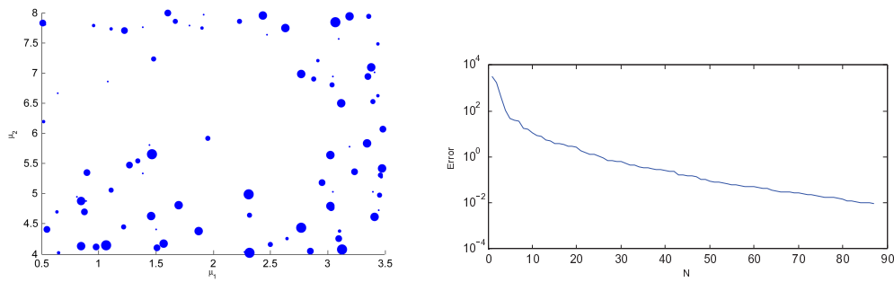
Figure 18: Added mass. Left: greedy (energy version) sample S_{N_{\max}} . Right: \max_{\mu \in \Xi_{\text{train}}} (\Delta_N^{\text{en}}(\mu) / \|\phi_N^{N_t}(\mu)\|_{\mu}) as a function of N for the Lagrange RB approximations associated with the sample of Fig. 18; here \Xi_{\text{train}} is a log-uniform random sample of size n_{\text{train}} = 3000 .
