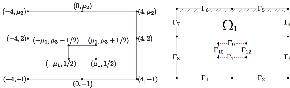
Figure 15: Parametrized geometry (left) and domain boundaries (right).
