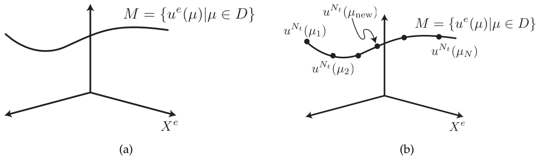
Figure 1: (a) Low-dimensional manifold on which the field variable resides and (b) approximation of a new solution at \mu_{new} with the “snapshots” u^{N_t}(\mu_n), 1 \leq n \leq N .
