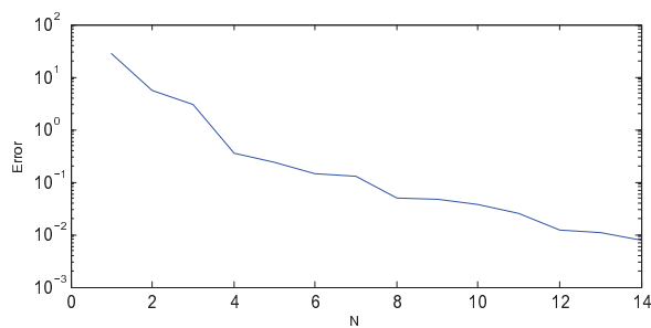
Figure 10: Venturi channel example: \max_{\mu \in \Xi_{\text{train}}} (\Delta_N^{\text{en}}(\mu) / \|\phi_N^{N_i}(\mu)\|_{\mu}) as a function of N for the Lagrange RB approximations associated with the sample of Fig. 9; here \Xi_{\text{train}} is a log-uniform random sample of size n_{\text{train}} = 3000 .
