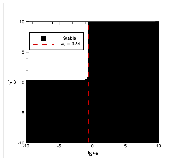
Figure 1: The stability region of the EIN-RK3-FC scheme corresponding to a_0 and \lambda for the linear convection-diffusion equation (2.11) with c = 0 . The scheme is stable when a_0 and \lambda are in the black region.
