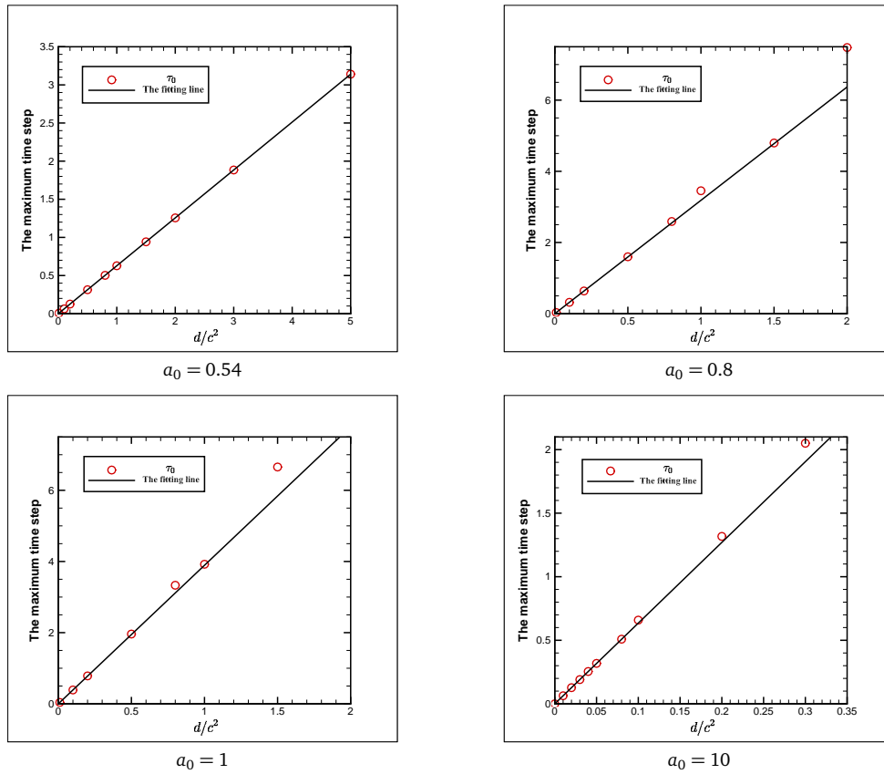
Figure 2: The maximum time step \tau_0 of the EIN-RK3-FC scheme corresponding to the diffusion coefficient d , the convection coefficient c and the stabilization parameter a_0 for the linear convection-diffusion equation (2.11).
