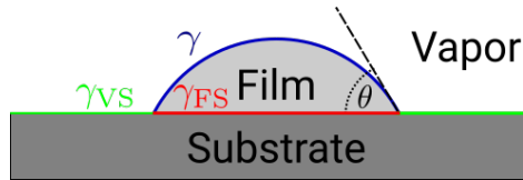
FIGURE 10. Young's law. The relation between (isotropic) film-vapor interface energy ( \gamma ), film-substrate interface energy ( \gamma_{FS} ) and the vapor-substrate interface energy ( \gamma_{VS} ) determines a unique wetting angle \theta .
