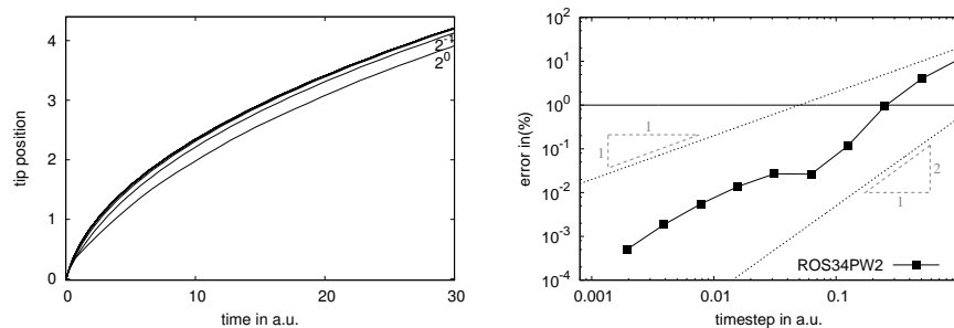
FIGURE 5. Rosenbrock ROS34WP2 convexity splitting scheme. (left) Tip position over time for various timesteps together with the reference solution (thick line). The numbers indicate the used timesteps. (right) Deviation from the reference solution over timesteps measured at t = 10 . The error has also been evaluated at t = 5 and t = 30 leading to similar behavior, not shown.
