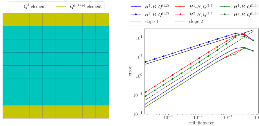
FIGURE 2. Convergence rates for a numerical approximation of (1) on a domain with periodic boundary conditions in the x direction and Dirichlet boundary conditions in the y direction. The grid on the left depicts which cells have been p -refined; the plot on the right shows convergence rates in the seminorms defined by Equations (2)-(3). The cyan cells have Q^1 (bilinear) shape functions; the yellow cells have been p -refined in the normal direction (i.e., they are P^m \otimes P^{m+p} elements, notated as Q^{(m,m+p)} ).
