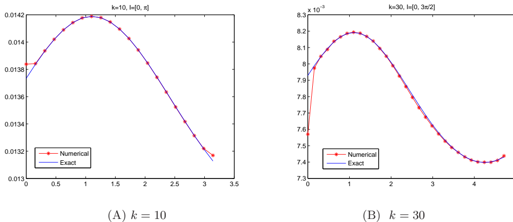
Fig. 5.4. Example 5.4: comparison between the numerical and the analytical solution.
