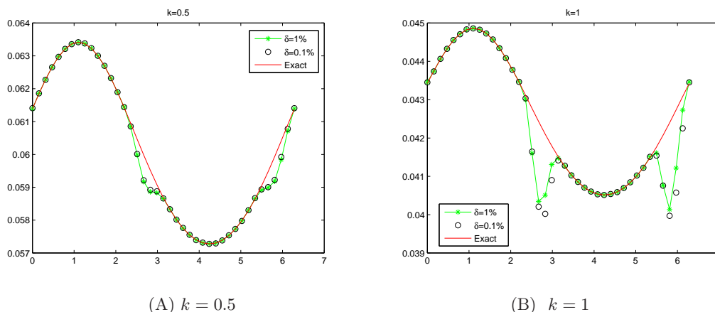
Fig. 5.3. comparison between the reconstructed wave field and the exact solution.
