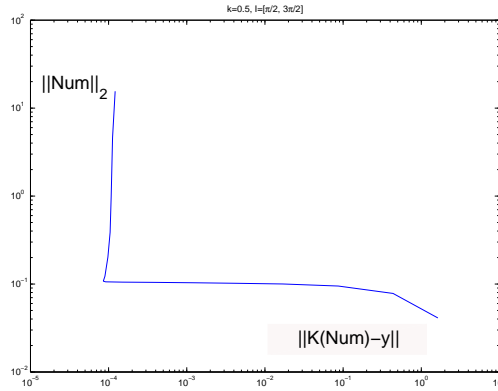
Fig. 5.1. Example 5.1: The L-curve obtained for \delta = 0 , k = 0.5 and I = [\pi/2, 3\pi/2] .
