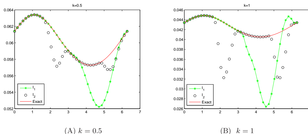
Fig. 5.2. Example 5.2: numerical results with different input.
