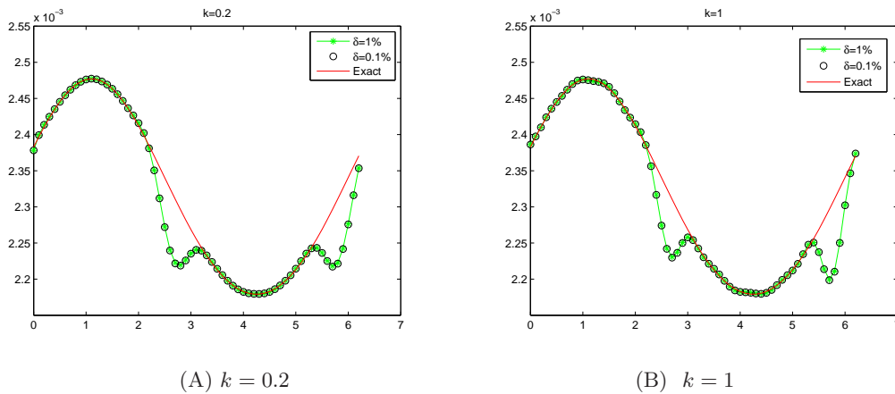
Fig. 5.6. Example 5.6: numerical results with different noises.
