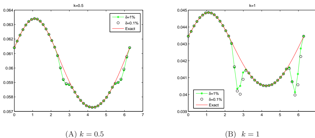
Fig. 5.3. comparison between the reconstructed wave field and the exact solution.
