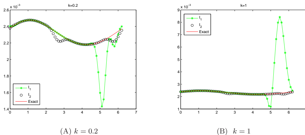
Fig. 5.5. Example 5.5: the reconstructed wave field and exact solution.
