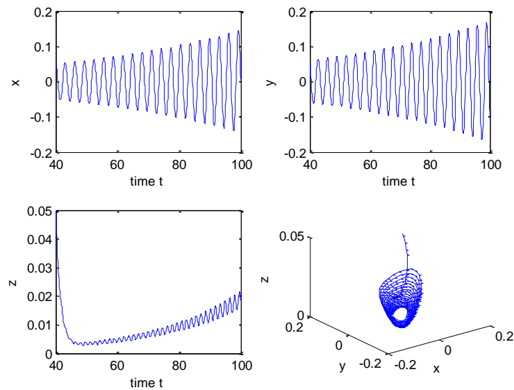
Fig. 3: The equilibrium E^* of the controlled system (13) is unstable when \tau_0 = 0.46 > 0.4483 .
