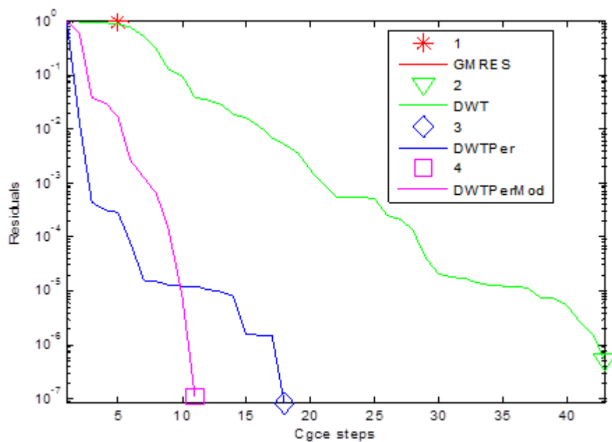
Fig. 2. Convergence of the fluid velocity y(x) using different schemes with Hartmann electric number ( Ha=1 ) and constant \alpha=0.5 & n=64 .
