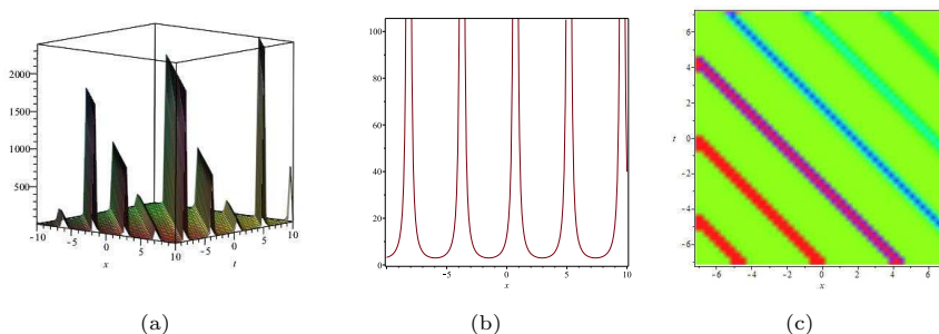
Figure 2. Singular periodic wave solution (3.5) for \alpha = -1, \beta = -1, \omega = 1, k = -1, b_2 = 1, a_1 = 2, c_1 = -0.5 . (a). 3-D plot; (b). the way of wave propagation along the x -axis; (c). Density plot.
