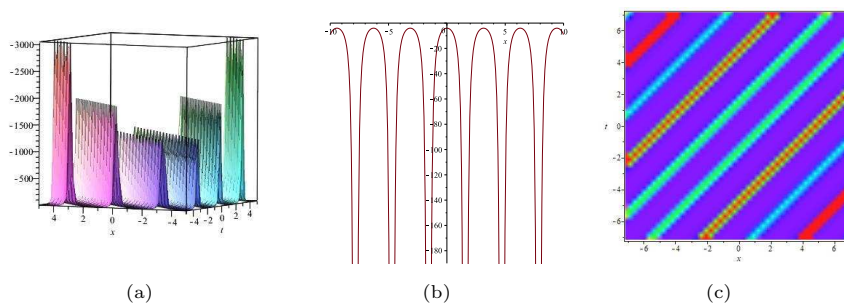
Figure 7. Singular periodic wave solution (5.6) for \alpha = 5 , \beta = 0.5 , \gamma = 1 , w = 1 . (a). 3-D plot; (b). The way of wave propagation along the x -axis; (c). Density plot.
