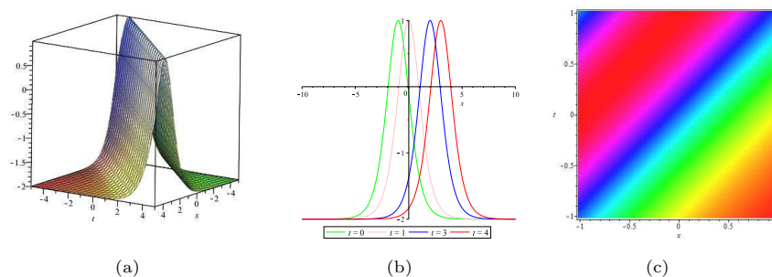
Figure 1. Bright-soliton solution (3.4) for \alpha = -1, \beta = 1, \omega = 1, k = 1, b_2 = 1, a_0 = -1, c_1 = 1 . (a). 3-D plot; (b). The way of wave propagation along the x -axis at different time; (c). Density plot.
