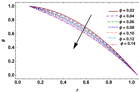
Figure 8: Temperature profile for fixed parameter are \alpha=0.02, \delta=0.11, \zeta=0.1, z=0.03, Rn=1, \epsilon=0.05, E_m=0.5, \sigma=0.1, G_r=1, B=6
