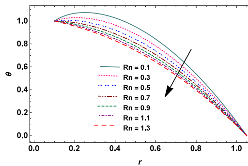
Figure 9: Temperature profile for fixed parameter are \alpha=0.02, \delta=0.11, \zeta=0.1, z=0.03, \phi=0.04, \epsilon=0.05, E_m=0.5, \sigma=0.1, G_r=1, B=4
