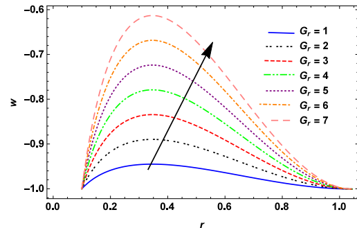
Figure 3: Velocity profile for fixed parameter are \alpha=0.02 , \delta=0.11 , B=0.17 , \phi=0.02 , z=0.08 , Rn=1 , \epsilon=0.05 , E_m=0.1 , \sigma=0.1 , \zeta=0.18
