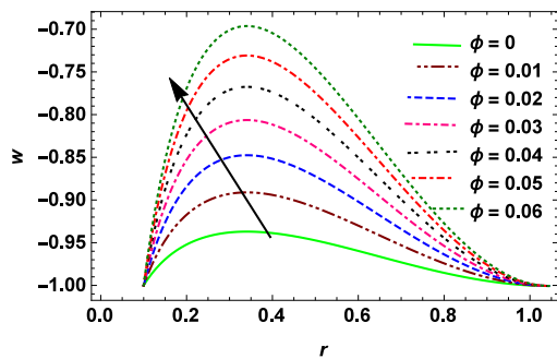
Figure 2: Velocity profile for fixed parameter are \alpha=0.02 , \delta=0.11 , B=0.17 , G_r=3 , z=0.08 , Rn=1 , \epsilon=0.05 , E_m=0.1 , \sigma=0.1 , \zeta=0.18
