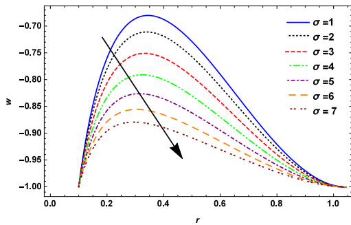
Figure 4: Velocity profile for fixed parameter are \alpha=0.02, \delta=0.11, B=0.17, \phi=0.02, z=0.08, Rn=1, \epsilon=0.05, E_m=0.1, G_r=6, \zeta=0.18
