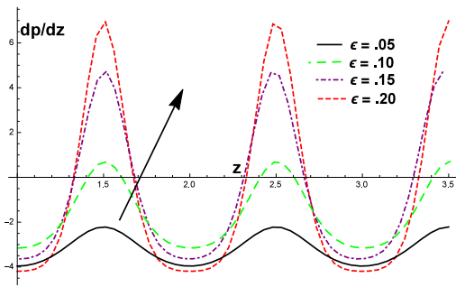
Figure 12: Pressure gradient for fixed parameter are \alpha=0.02 , \zeta=0.1 , \delta=0.11 , \phi=0.02 , \sigma=0.01
