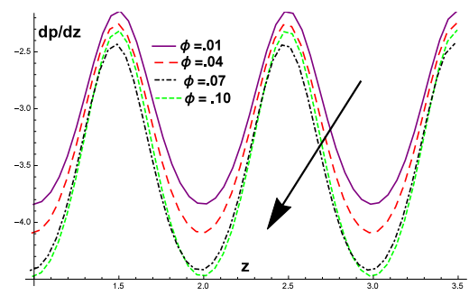
Figure 11: Pressure gradient for fixed parameter are \alpha=0.02 , \zeta=0.1 , \delta=0.11 , \sigma=0.01 , \epsilon=0.05
