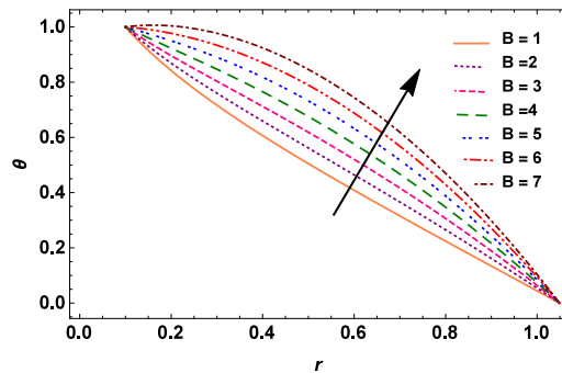
Figure 7: Temperature profile for fixed parameter are \alpha=0.02, \delta=0.11, \Phi=0.02, \zeta=0.1, z=0.03, Rn=1, \epsilon=0.05, E_m=0.5, \sigma=0.1, G_r=1
