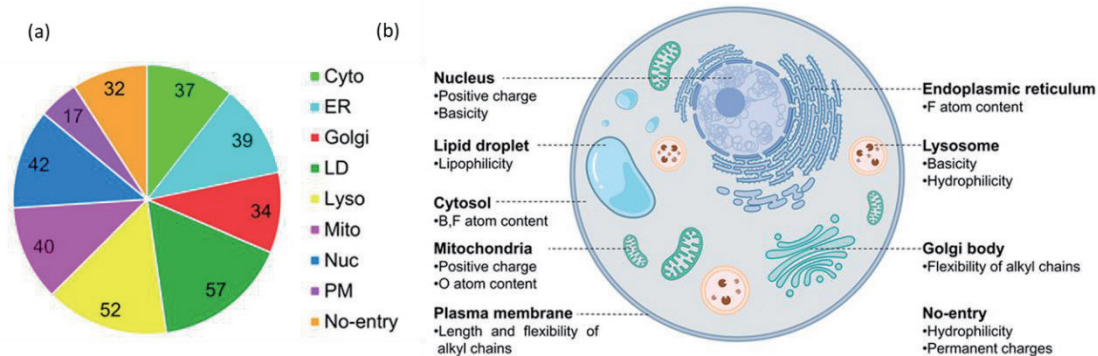
Figure 6. (a) Classification into 9 target organelles for database containing 350 fluorescent probes. (b) A visual representation of significant characteristics of probes that influence their localization, acquired through MDI analysis of the model. Copyright (2023) Multidisciplinary Digital Publishing Institute.
